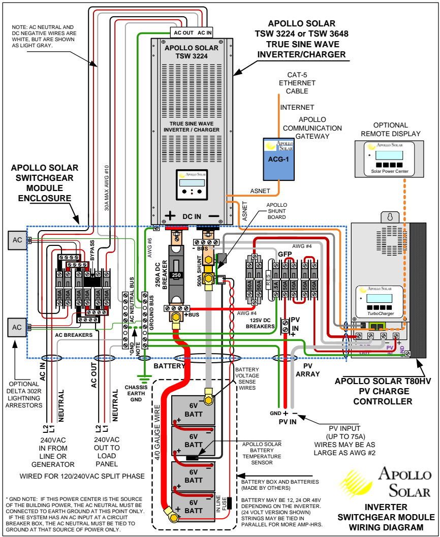
Wiring Diagram of the ISM 120/240 with T80HV Charge Controller
